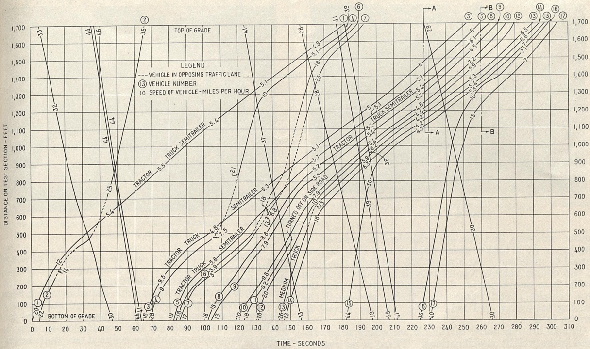
FIGURE 1.—TIME-DISTANCE CURVES SHOWING PROGRESS OF VEHICLES THROUGH TEST SECTION. CURVES SLOPING TO RIGHT INDICATE VEHICLES ASCENDING THE HILL; CURVES SLOPING TO LEFT INDICATE DESCENDING VEHICLES. ORDINATE BETWEEN ANY TWO CURVES INDICATES DISTANCE IN FEET BETWEEN FRONT AXLES OF RESPECTIVE VEHICLES. VEHICLES NOS. 1, 3, 5, AND 8 ARE TRACTOR TRUCK SEMITRAILER COMBINATIONS; VEHICLE NO. 13 IS A MEDIUM TRUCK; ALL OTHER VEHICLES ARE PASSENGER CARS.
