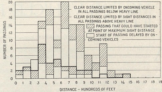
FIGURE 11.—MAXIMUM DISTANCE THAT DRIVERS OF PASSING VEHICLES COULD SEE THAT LEFT LANE WAS FREE OF ONCOMING TRAFFIC AT THE TIME PASSING MANEUVERS WERE COMPLETED. (INCLUDING ONLY THOSE VEHICLES THAT SLOWED DOWN TO SAME SPEED AS VEHICLES TO BE PASSED PRIOR TO STARTING THE PASSING MANEUVERS ON STUDY SECTION.)
