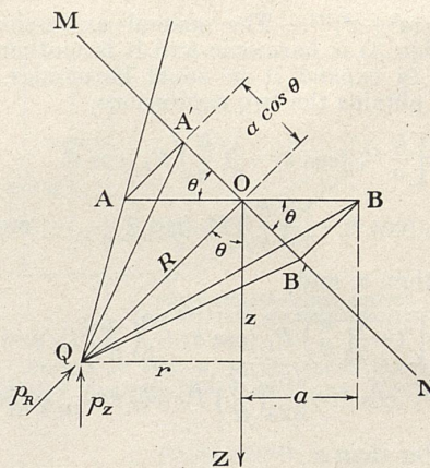
FIGURE 3.—THE PROJECTION OF THE LOADED CIRCULAR AREA, AB , IN THE HORIZONTAL PLANE ON THE PLANE MN IS AN ELLIPSE WITH MINOR AXIS A'B' AND MAJOR AXIS AB .
