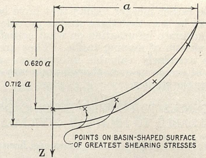
FIGURE 4.—POINTS AT WHICH THE STRESSED MATERIAL UNDER A UNIFORMLY LOADED CIRCULAR AREA WOULD BE MOST LIKELY TO FAIL.
