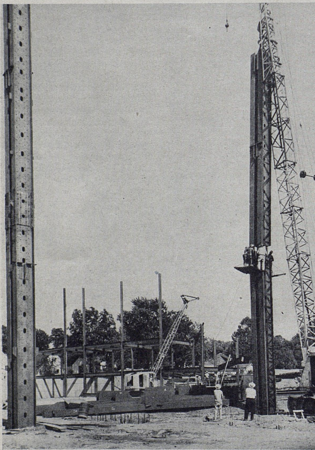
Steel work is now going up on the University's Memorial Auditorium Field House, and a long-time dream of Kentucky alumni and students is being realized. Pictured here is the first view of columns and crossbeams showing the beginning of the steel skeleton construction. The best estimate as the final completion date is "early 1950."
