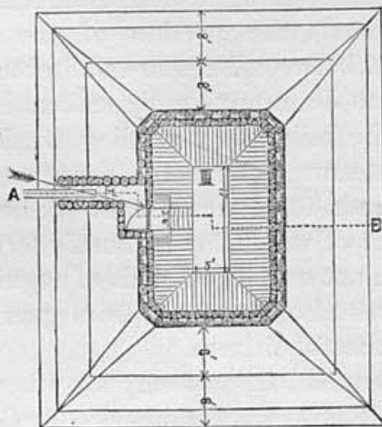
FIG. 1. PLAN OF RECTANGULAR BLOCK-HOUSE.
