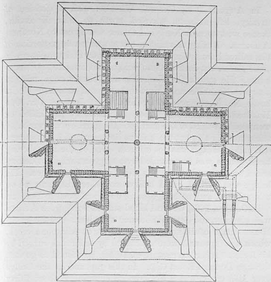
FIG. 7. PLAN OF ARTILLERY BLOCK-HOUSE.
