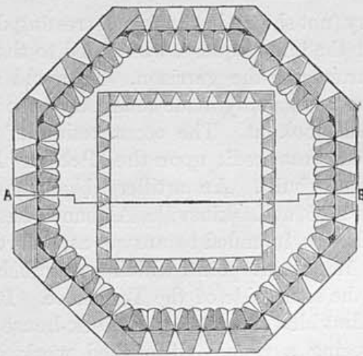
FIG. 5. PLAN OF OCTAGONAL BLOCK-HOUSE WITH TOWER.
