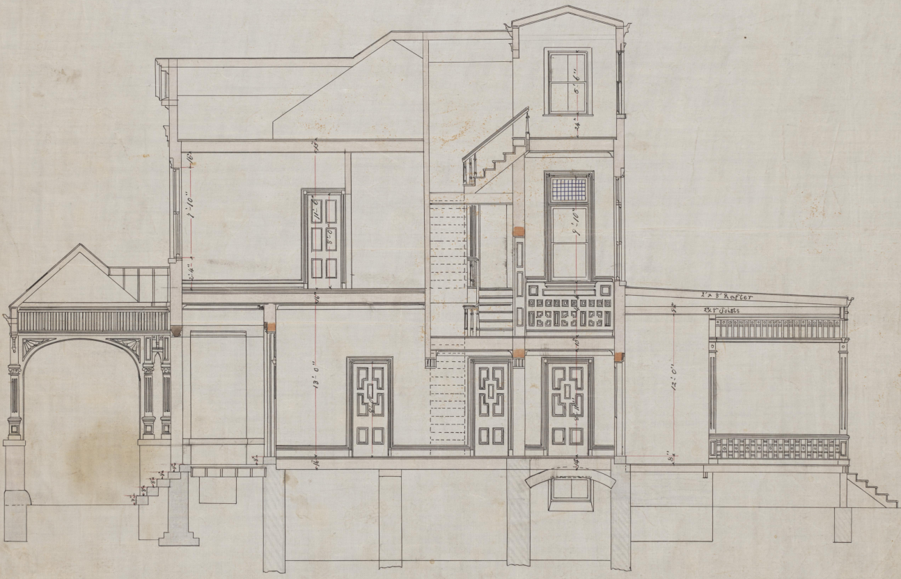
TRANSVERSE SECTION
