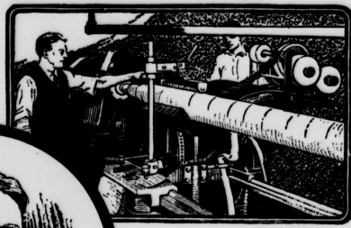
Winding high voltage insulation, 1921 — 220,000 Volts
