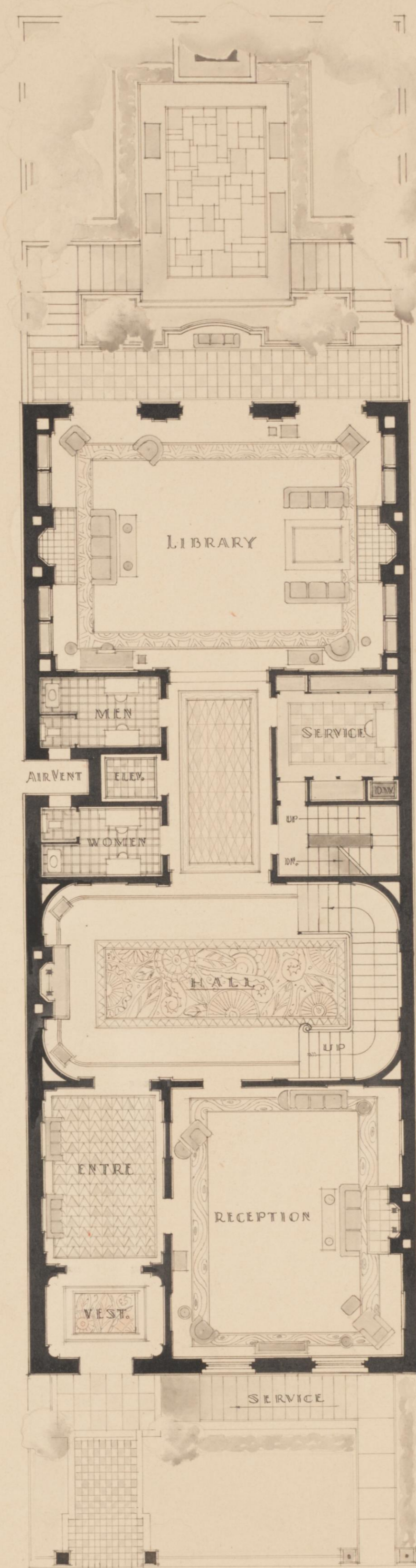
FIRST FLOOR
