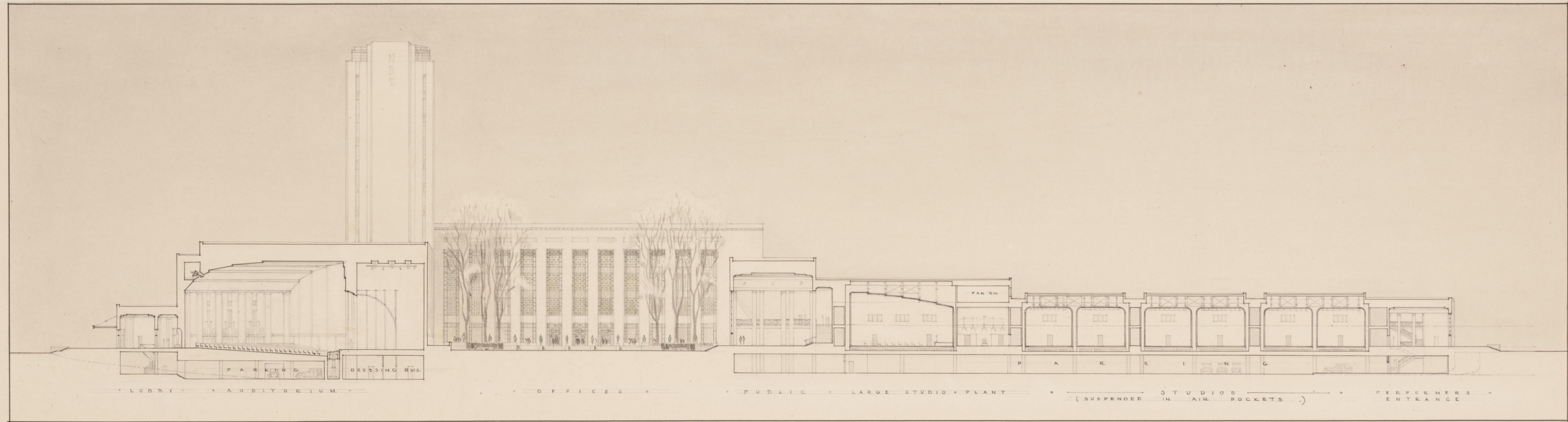
L O N G I T U D I N A L S E C T I O N SCALE ONE INCH EQUALS THIRTY TWO FEET.
