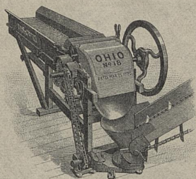
"OHIO" SELF-FEED ENSILAGE CUTTER.
