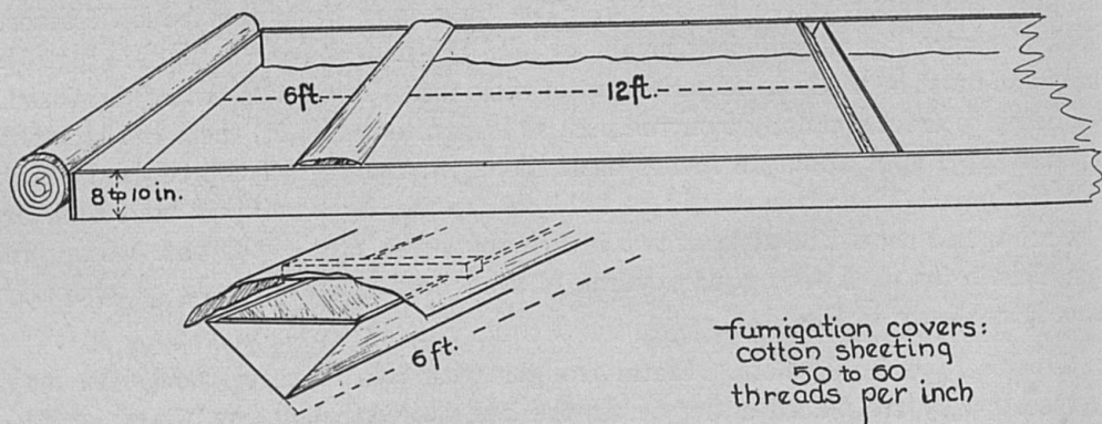
Fig. 6.—Plan of trough evaporators with covers, and the arrangement of these troughs used in fumigating with benzol.
