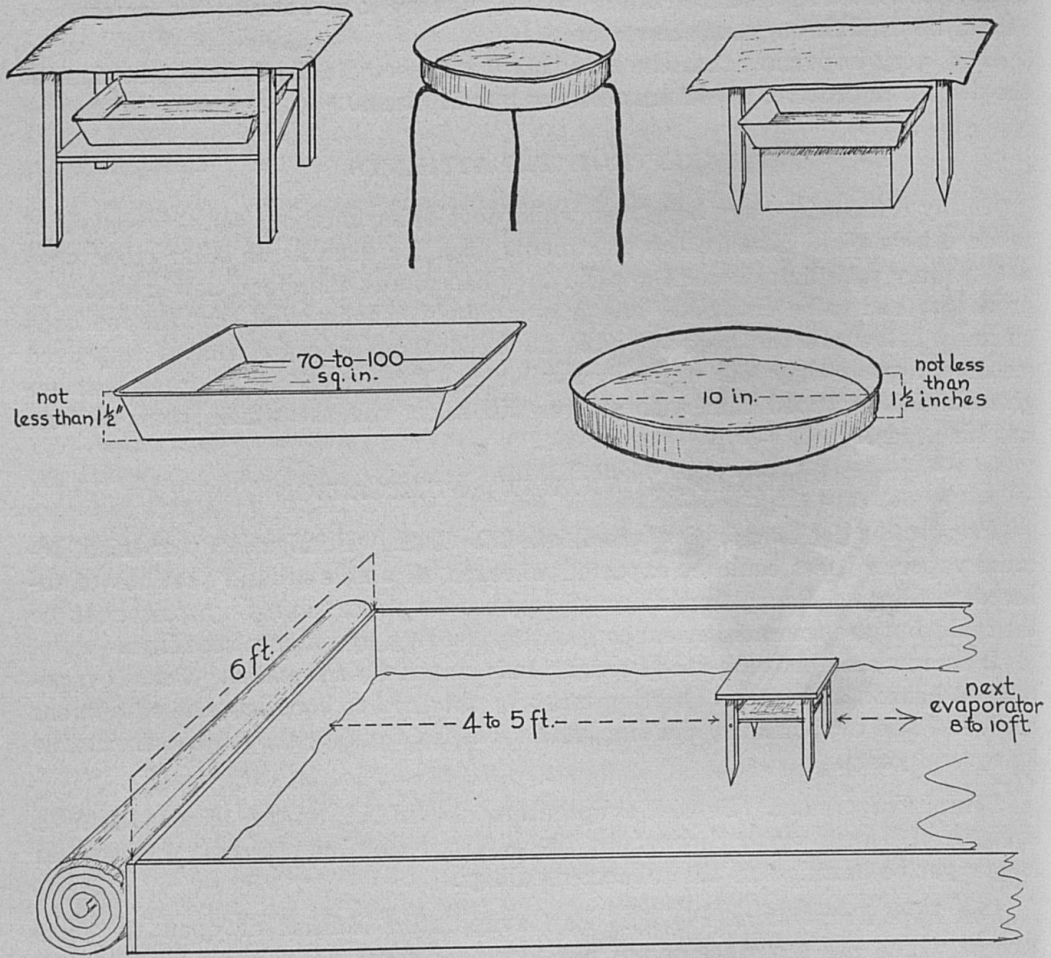
Fig. 5.—Plan showing evaporators, stands, covers, and spacing of evaporators within the seed-bed used in fumigating with benzol.
