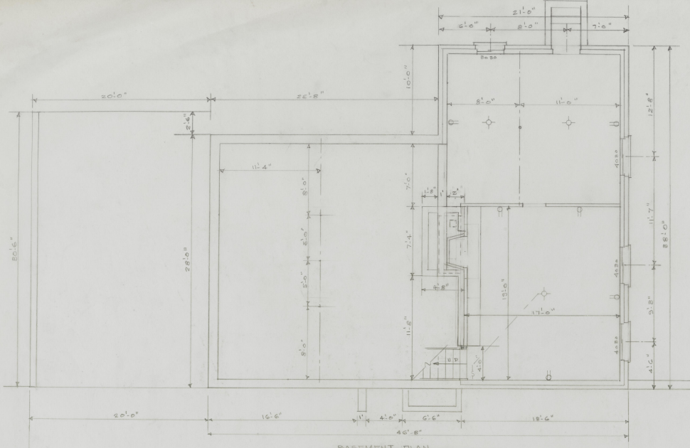
BASEMENT PLAN
