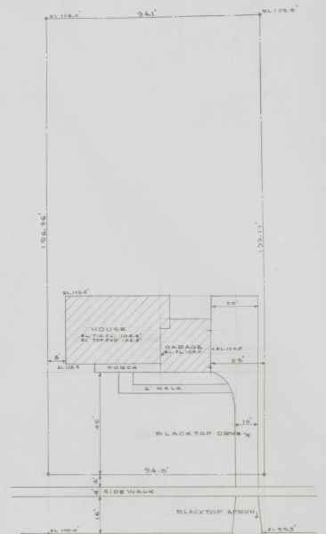
PLOT PLAN SCALE 1"=20'
