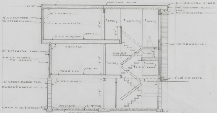
TYPICAL SECTION SCALE 1/4" = 1'-0"
