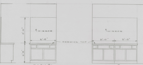
VANITIES SCALE 1/2" = 1'-0"
