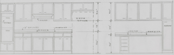
KITCHEN CABINETS SCALE 1/2" = 1'-0"
