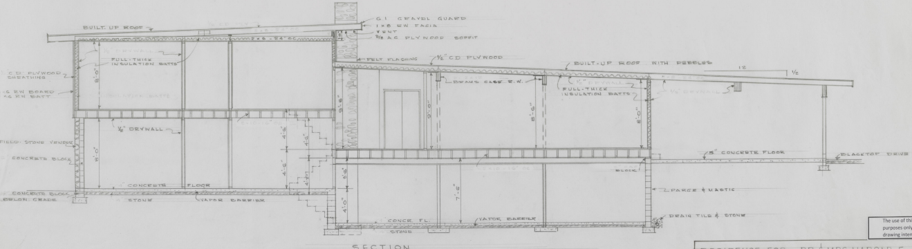
SECTION
