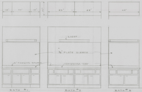
BATH VANITIES SCALE 1/4\"/>
