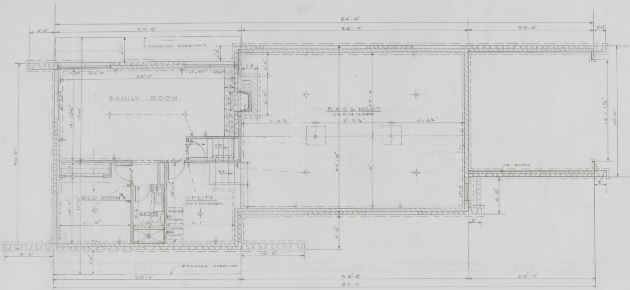
PLAN - LOWER LEVEL
