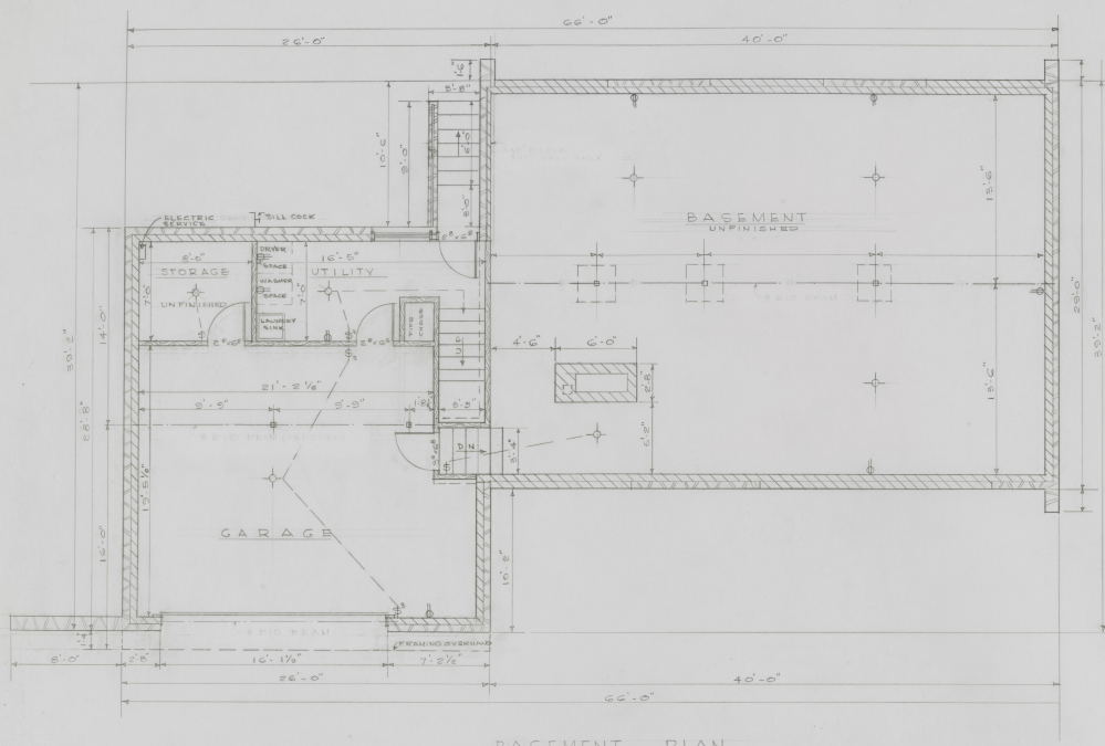
BASEMENT PLAN
