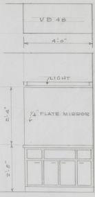
VANITIES BATH #1 BATH #2 SCALE 1/2" = 1'-0"
