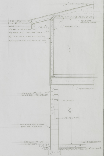
BEDROOM SECTION SCALE 1/4" = 1'-0"
