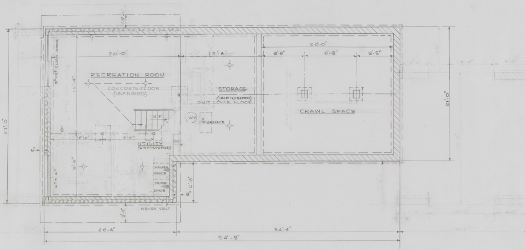
FOUNDATION PLAN
