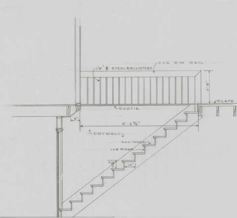
STAIR SECTION
