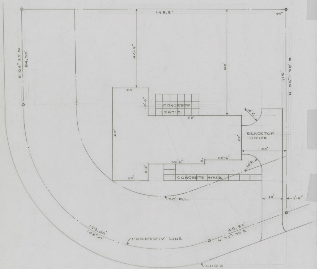
PLOT PLAN SCALE 1" = 16'-0"
