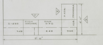
PLAN - KITCHEN CABINETS
