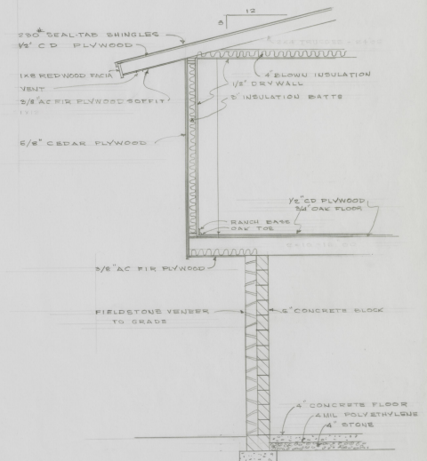
TYPICAL WALL SECTIONS SCALE 1/2" = 1'-0"
