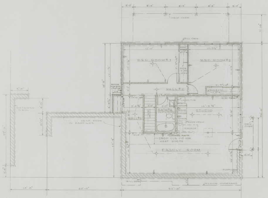
PLAN LOWER FLOOR
