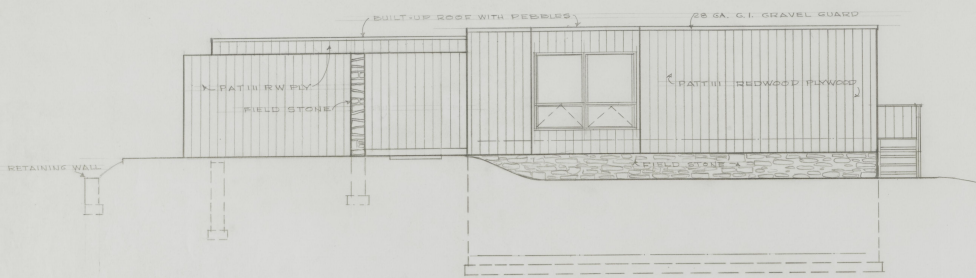
FRONT ELEVATION
