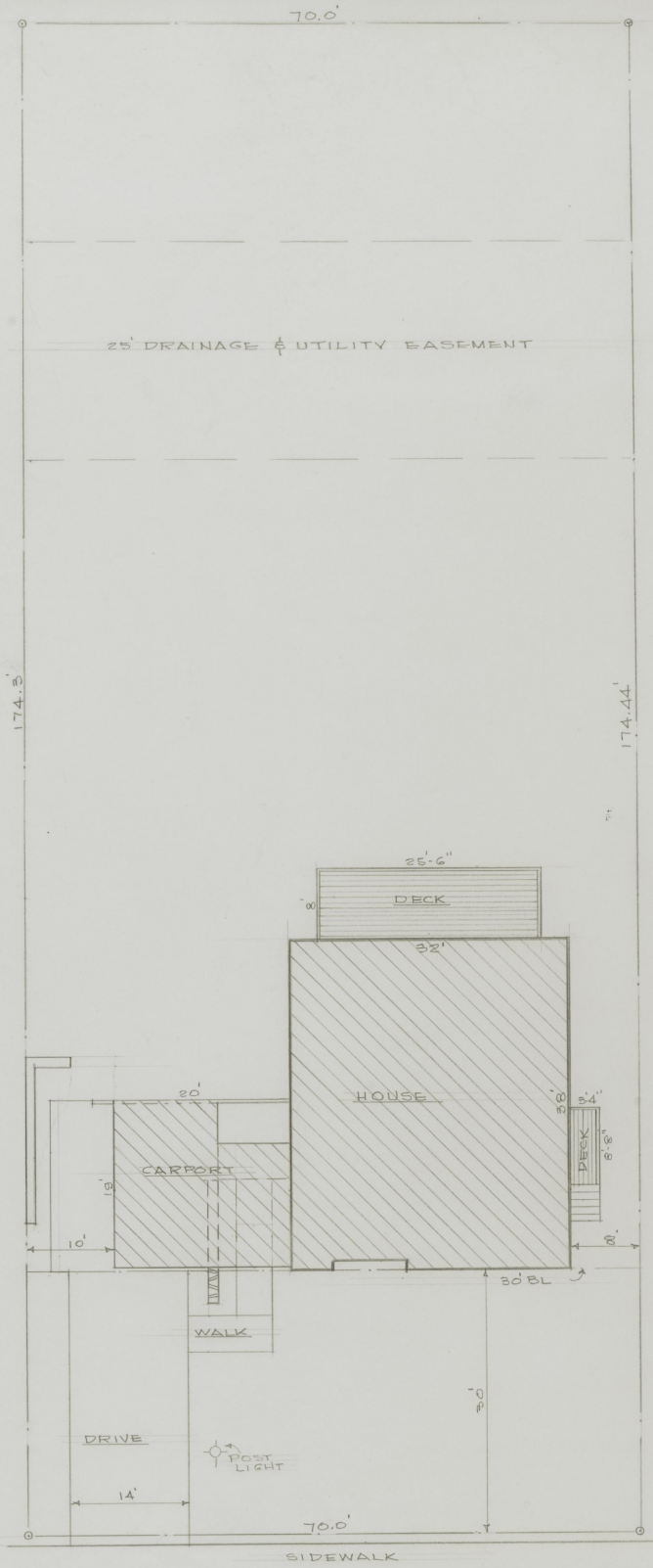
PLOT PLAN - LOT 8, BLOCK A, UNIT 5, GAINSWAY SUB. SCALE 1" = 10'
