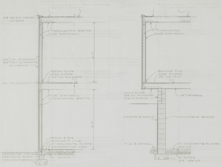
TYPICAL WALL SECTIONS SCALE 1/2" = 1'-0"
