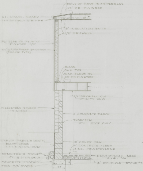
TYPICAL SECTION SCALE: 1/2" = 1'-0"
