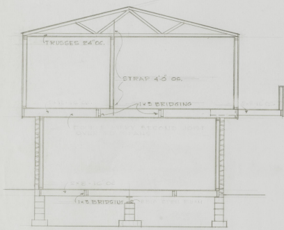
TYPICAL SECTION
