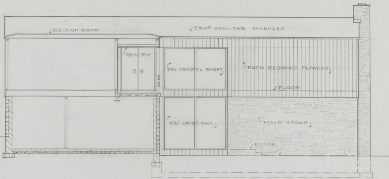
FRONT ELEVATION & SECTION AA
