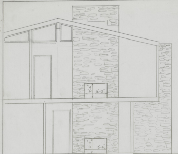
FIREPLACE ELEVATION
