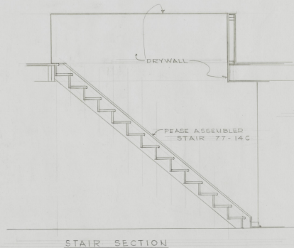
STAIR SECTION
