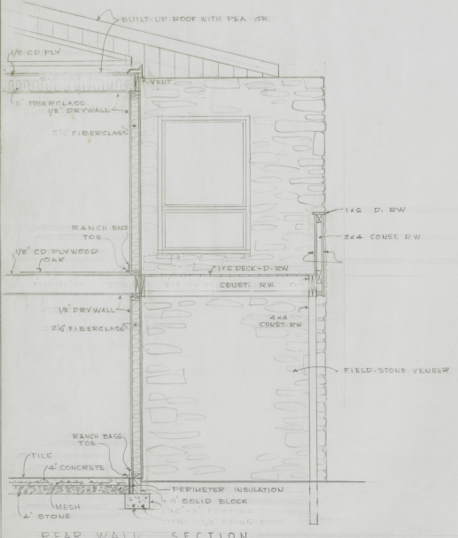
REAR WALL SECTION
