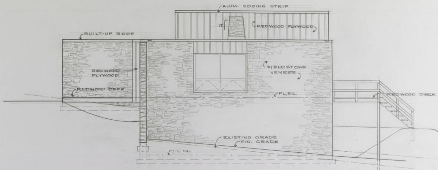
RIGHT SIDE ELEVATION 1/4" = 1'-0"
