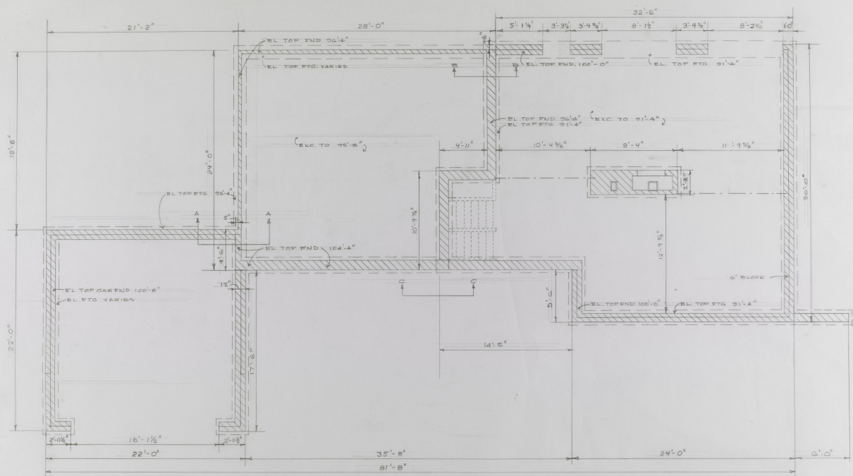
FOUNDATION PLAN 1/4" = 1'-0"
