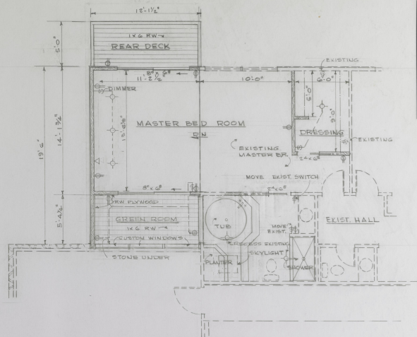
PLAN - UPPER LEVEL 1/4" = 1'-0"
