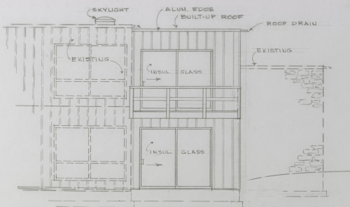
REAR ELEVATION 1/4" = 1'-0"
