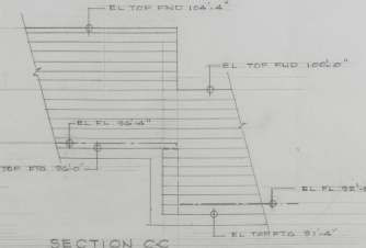
SECTION C-C 1/4" = 1'-0"
