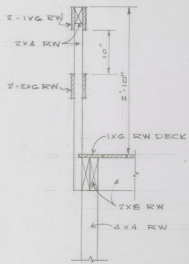
DECK RAIL DETAIL 1" = 1'-0"
