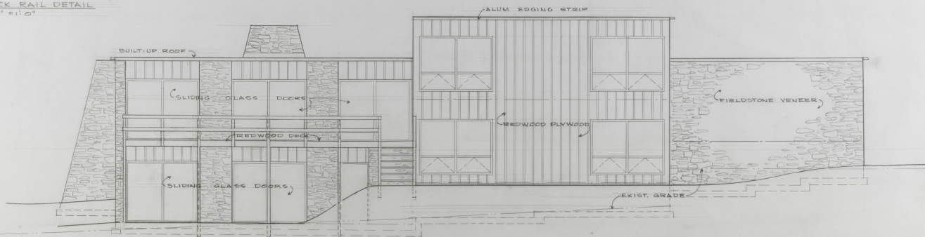
REAR ELEVATION 1/4" = 1'-0"
