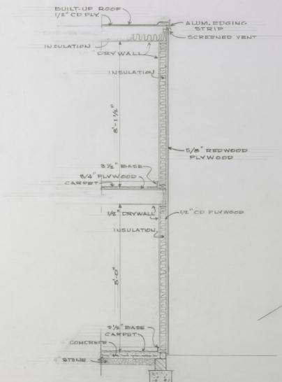
SECTION-REAR WALL BEDROOM 1/2" = 1'-0"
