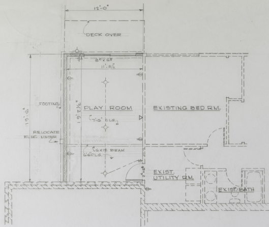
PLAN - LOWER LEVEL 1/4" = 1'-0"
