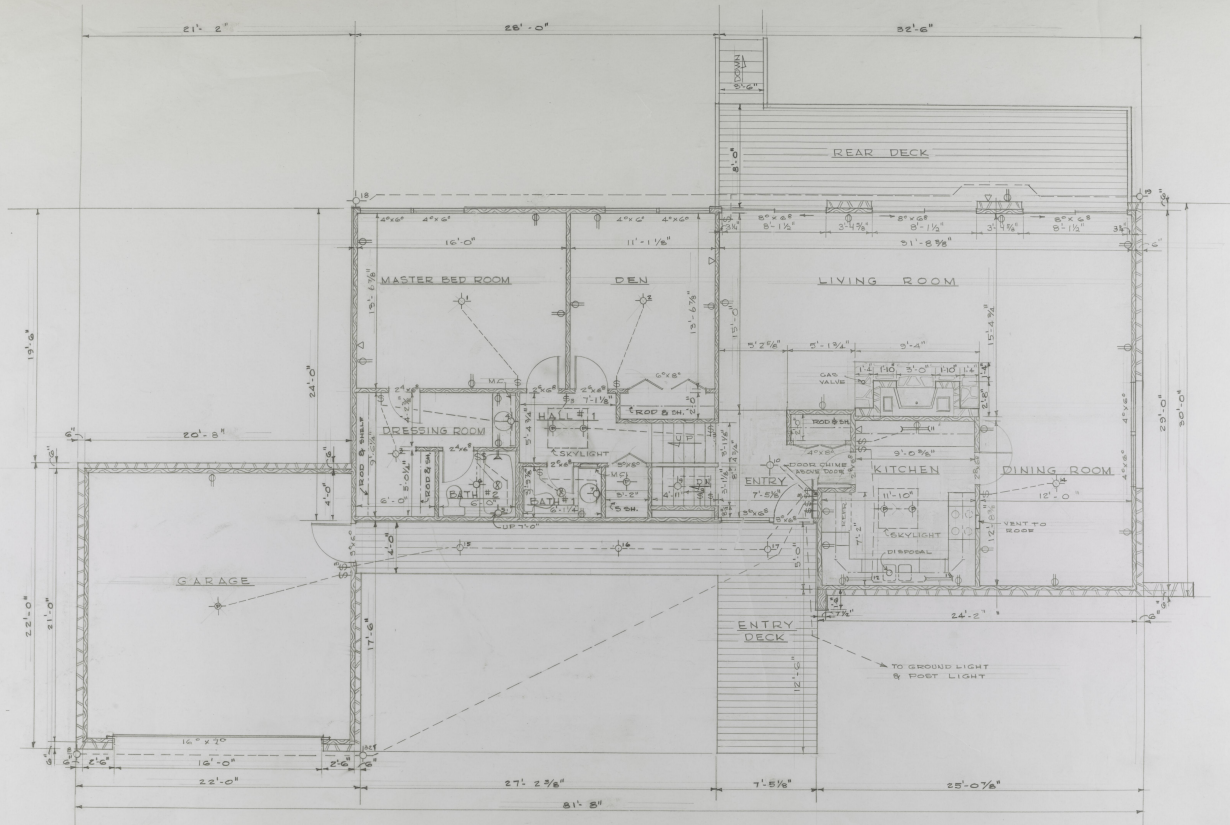
PLAN - UPPER LEVEL 1/4" = 1'-0"
