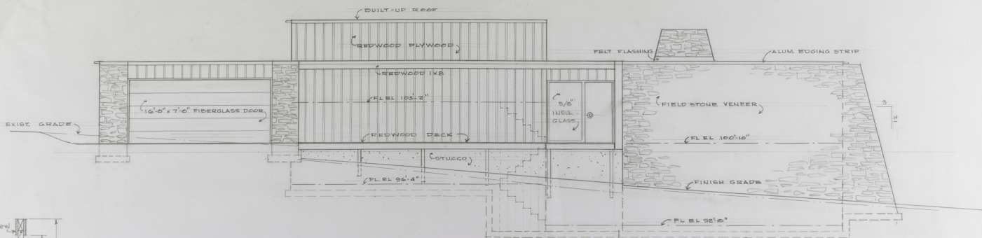
FRONT ELEVATION 1/4" = 1'-0"
