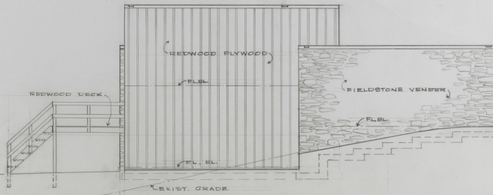
LEFT SIDE ELEVATION 1/4" = 1'-0"
