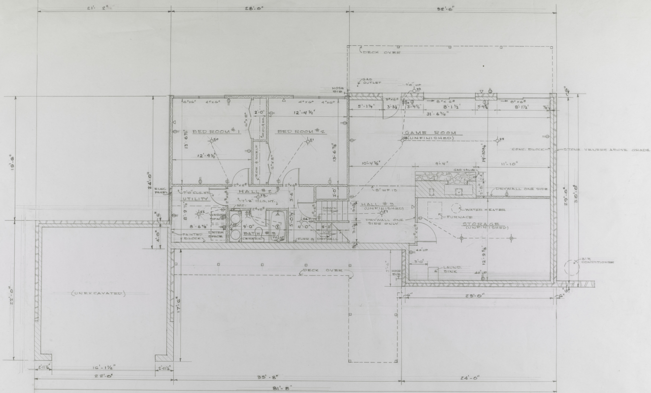
PLAN - LOWER LEVEL 1/4" = 1'-0"
