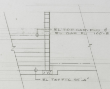
SECTION A-A 1/4" = 1'-0"
