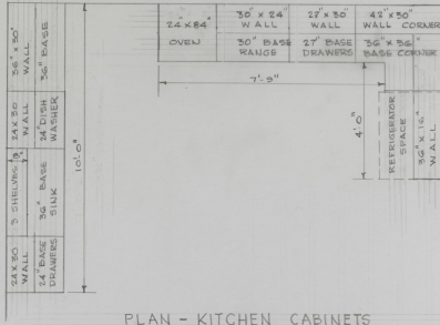
PLAN - KITCHEN CABINETS 1/2" = 1'-0"
