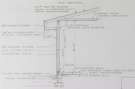
TYPICAL SECTION-REAR WALL 1/2" = 1'-0"
