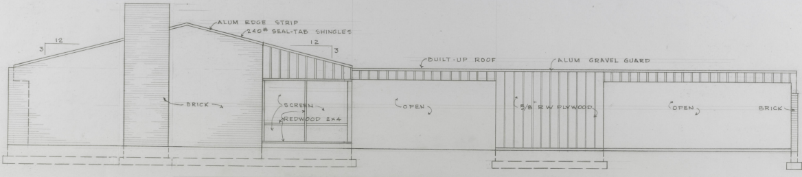
LEFT SIDE ELEVATION 1/4" = 1'-0"
