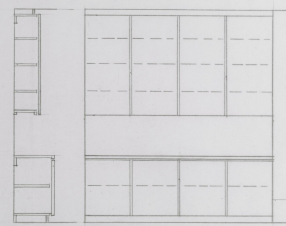
FAMILY ROOM CABINET 1/2" = 1'-0"
