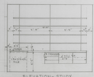
ELEVATION-STUDY 1/2" = 1'-0"
