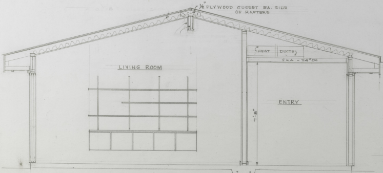
LIVING ROOM SECTION 1/2" = 1'-0"
