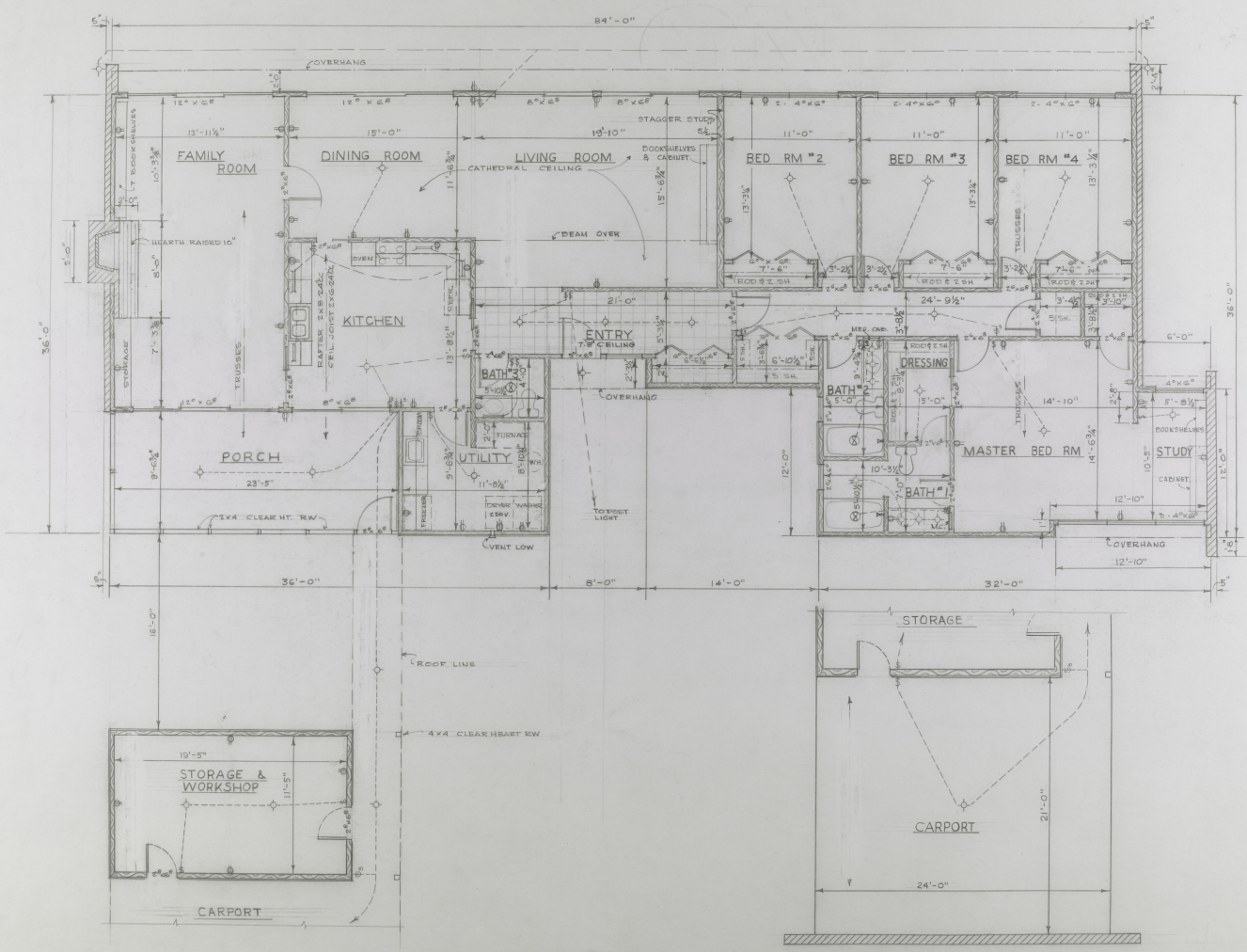
PLAN 1/4" = 1'-0"
