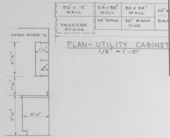
SECTION 1/2" = 1'-0"
