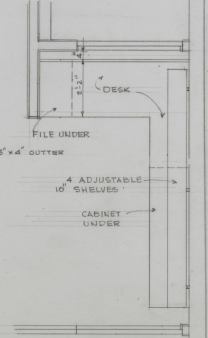
PLAN-STUDY DESK 1/2" = 1'-0"
