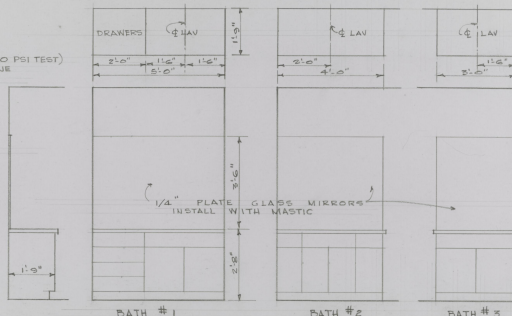
VANITY ELEVATIONS 1/2" = 1'-0"
