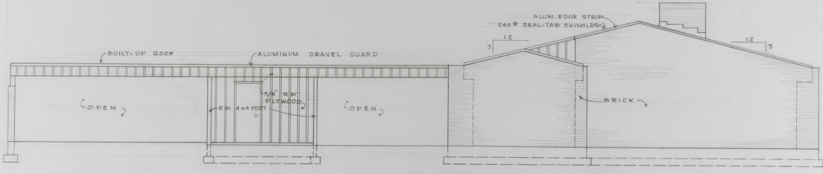
RIGHT SIDE ELEVATION 1/4" = 1'-0"
