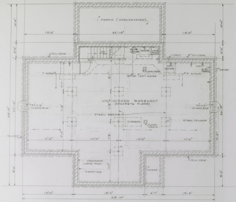
BASEMENT PLAN
