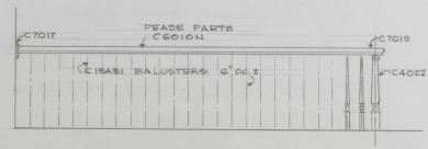
STAIR RAIL 1/2" = 1'-0"
