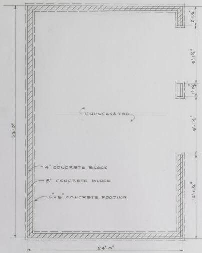
GARAGE - FOUNDATION PLAN
