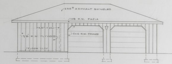
GARAGE-RIGHT SIDE ELEVATION 1/4" = 1'-0"
