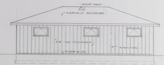
GARAGE-LEFT SIDE ELEVATION 1/4" = 1'-0"
