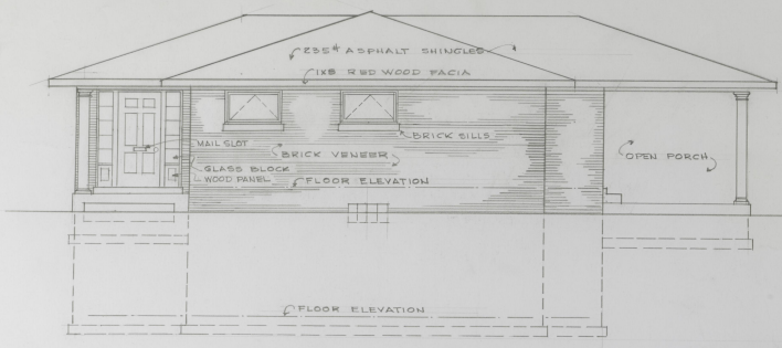
RIGHT SIDE ELEVATION 1/4" = 1'-0"
