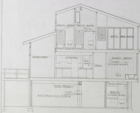
KITCHEN SECTION 1/4" = 1'-0"
