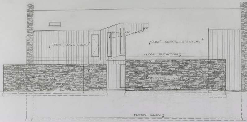
FRONT ELEVATION 1/4" = 1'-0"
