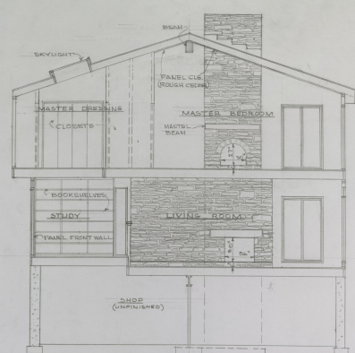
LIVING ROOM SECTION 1/4" = 1'-0"
