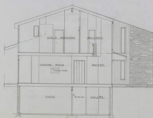
DINING ROOM SECTION 1/4" = 1'-0"
