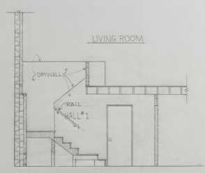
STAIR SECTION 1/4" = 1'-0"
