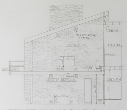
SECTION-FIREPLACE WALL ELEVATION (REAR) 1/4" = 1'-0"
