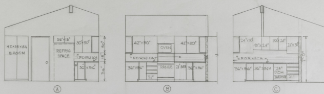
ELEVATIONS 1/4" = 1'-0"
