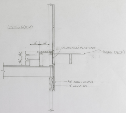
LIVING ROOM- REAR DECK DETAIL 3/4" = 1'-0"
