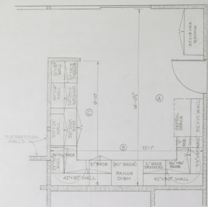
PLAN 1/4" = 1'-0"
