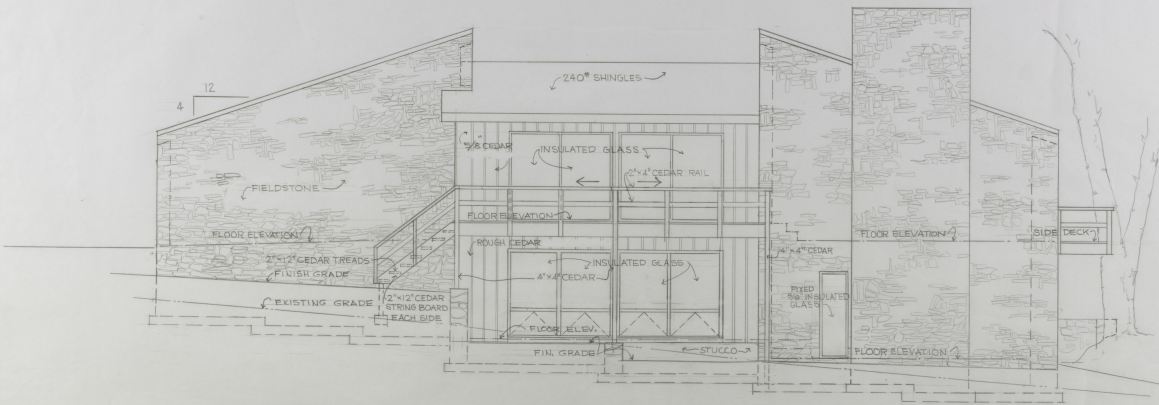
REAR ELEVATION 1/4" = 1'-0"
