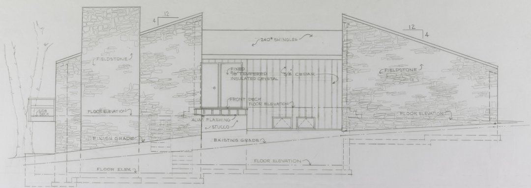
FRONT ELEVATION 1/4" = 1'-0"
