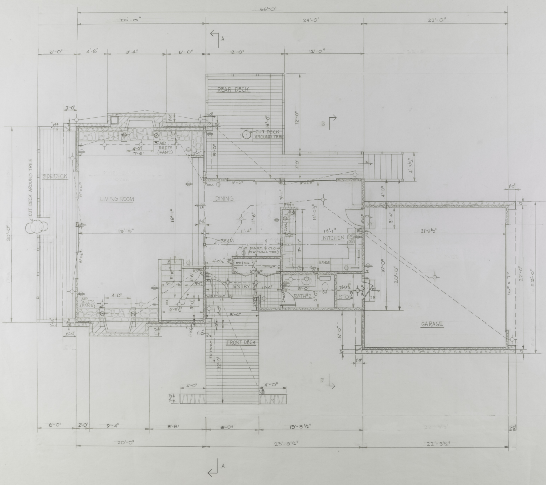
PLAN 1/4" = 1'-0"
