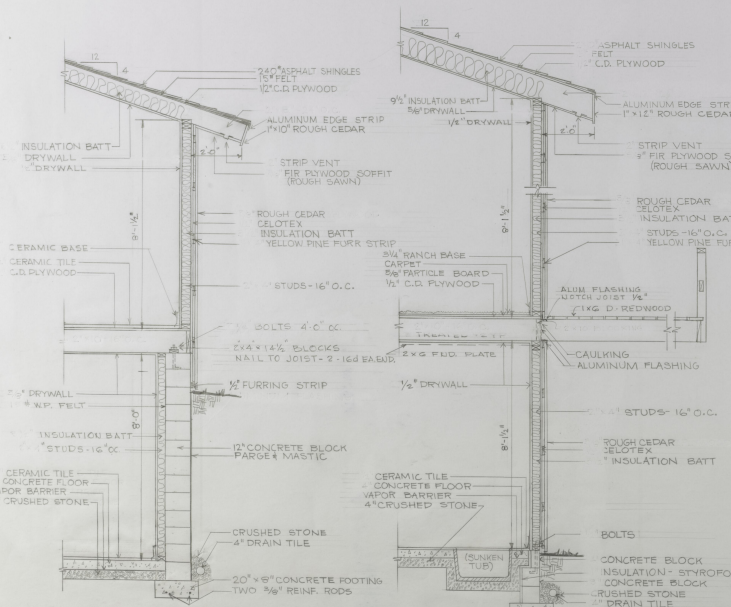
BATH #2-BATH #1 WALL SECT 1/2" = 1'-0"
