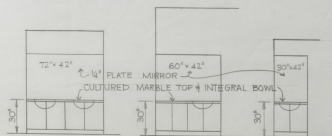
ELEVATIONS 1/4" = 1'-0"
