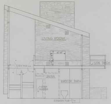
SECTION-FIREPLACE WALL ELEVATION (FRONT) 1/4" = 1'-0"
