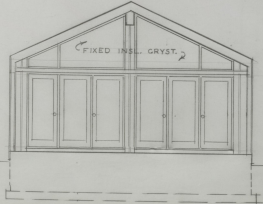
PORCH ELEVATION 1/4" = 1'-0"
