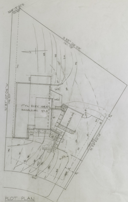
PLOT PLAN LOT 35 UNIT 3 THE WOODS LANDSDOWNE MERRICK UNIT 17A SCALE 1/4" = 1'-0"
