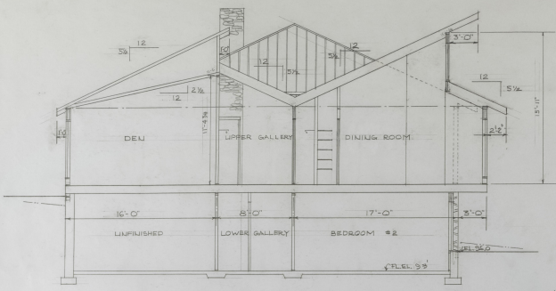
DINING ROOM SECTION 1/4" = 1'-0"
