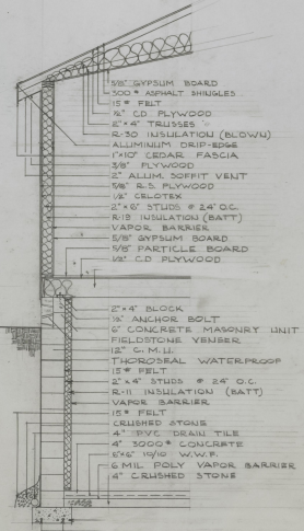
TYPICAL SECTION 1/8" = 1'-0"
