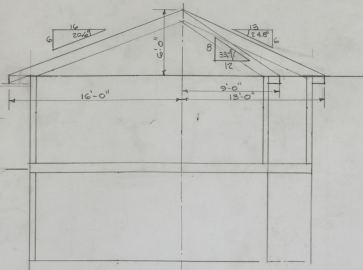
ROOF SECTION 1/4" = 1'-0"
