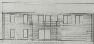
REAR ELEVATION 1/8" = 1'-0"
