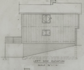
LEFT SIDE ELEVATION SCALE 1/8" = 1'-0"
