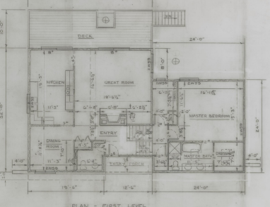
PLAN - FIRST LEVEL SCALE 1/8" = 1'-0"
