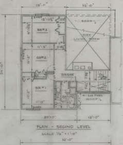
PLAN - SECOND LEVEL SCALE 1/8" = 1'-0"
