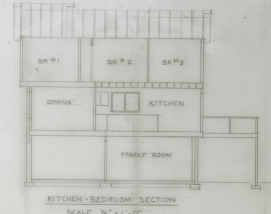
KITCHEN-BEDROOM SECTION SCALE 1/8" = 1'-0"
