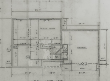
PLAN - LOWER LEVEL SCALE 1/8" = 1'-0"
