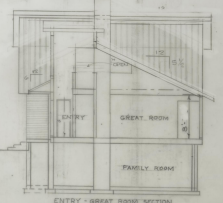
ENTRY-GREAT ROOM SECTION SCALE 1/8" = 1'-0"
