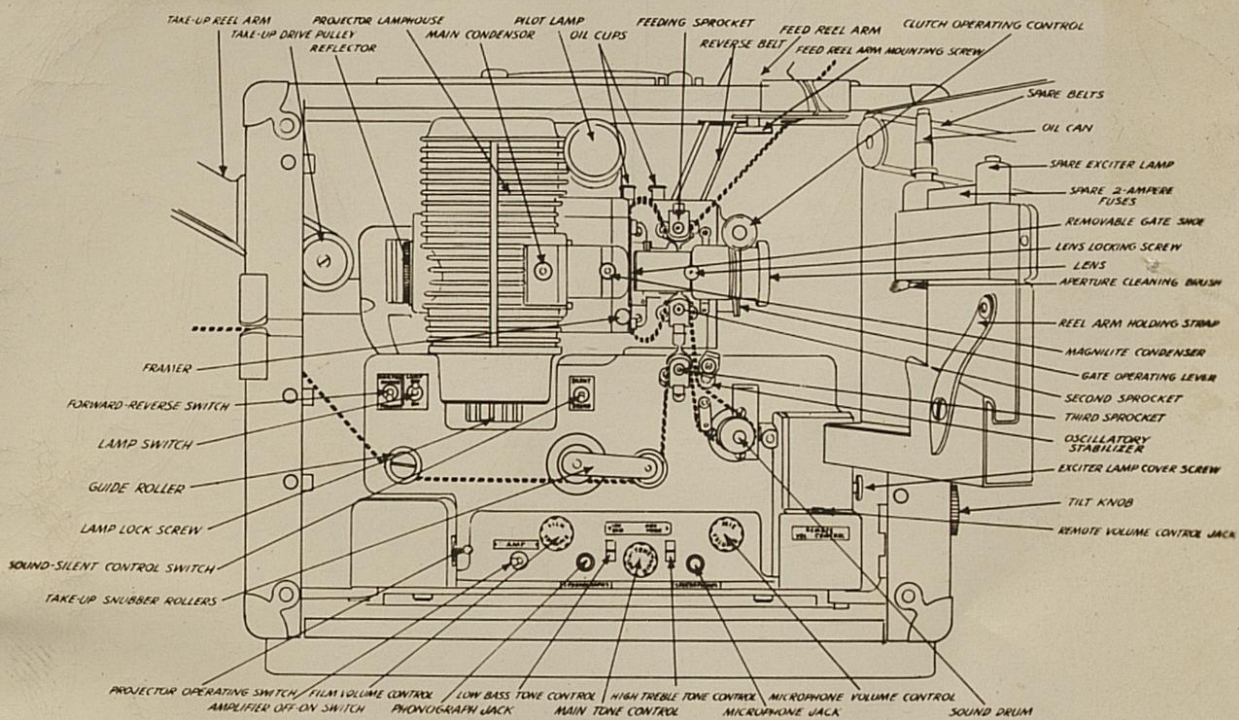
BELL & HOWELL COMPACT "UTILITY" MODEL - FILMOSOUND 16MM.
