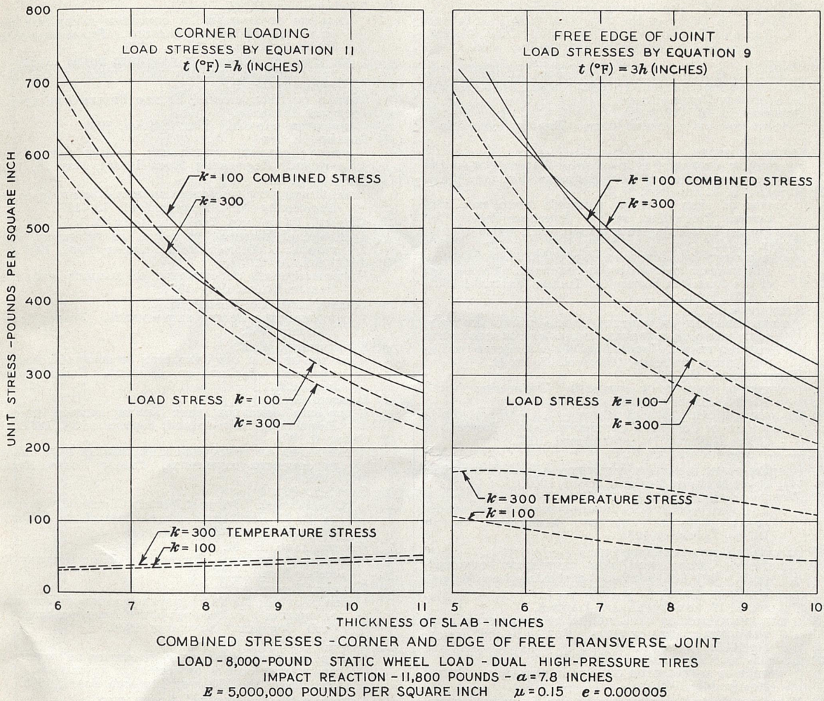
FIGURE 17.—EFFECT OF SLAB THICKNESS AND SUBGRADE MODULUS ON COMBINED STRESSES DUE TO LOAD AND TEMPERATURE WARPING IN THE CORNER AND EDGE OF A FREE TRANSVERSE JOINT IN A SLAB 10 FEET WIDE.
