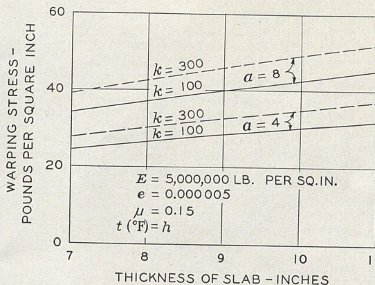
FIGURE 13.—TEMPERATURE-WARPING STRESSES, CORNER OF SLAB.
