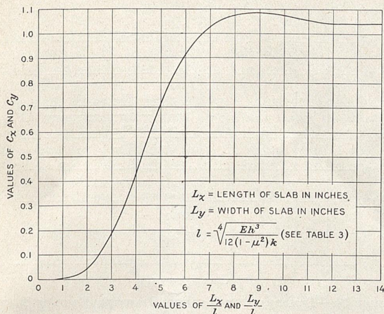
FIGURE 10.—COEFFICIENTS FOR WARPING STRESSES DUE TO TEMPERATURE.
