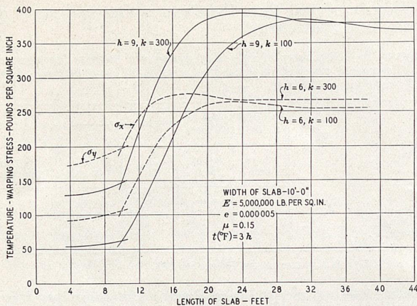
FIGURE 11.—TEMPERATURE-WARPING STRESSES, INTERIOR OF SLAB.
