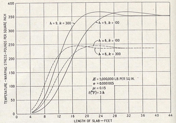
FIGURE 12.—TEMPERATURE-WARPING STRESSES, EDGE OF SLAB.
