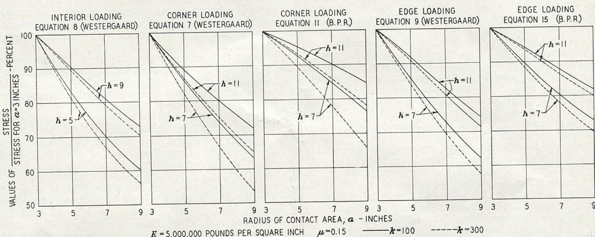
FIGURE 6.—EFFECT ON COMPUTED STRESSES OF VARIATIONS IN RADIUS OF CONTACT AREA, a .
