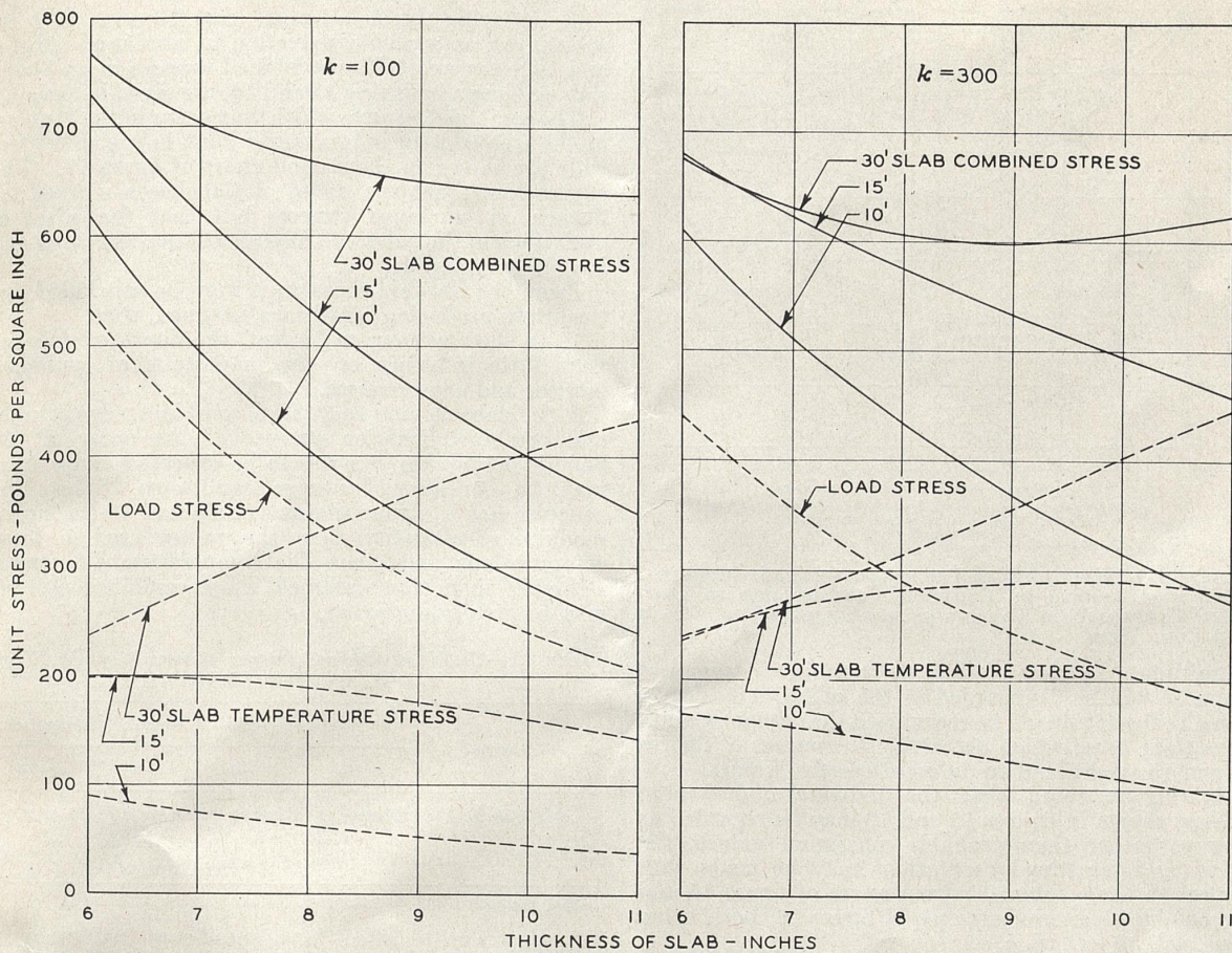
COMBINED STRESSES - EDGE LOADING - EDGES WARPED DOWN (DAY)
