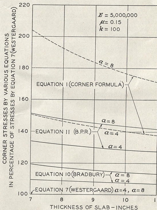
FIGURE 1.—COMPARISON OF CORNER STRESSES COMPUTED BY VARIOUS EQUATIONS.
