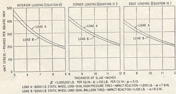
FIGURE 9.—COMPARISON OF STRESSES DUE TO 8,000-POUND WHEEL LOAD ON HIGH-PRESSURE TIRES AND 9,000-POUND WHEEL LOAD ON BALLOON TIRES.
